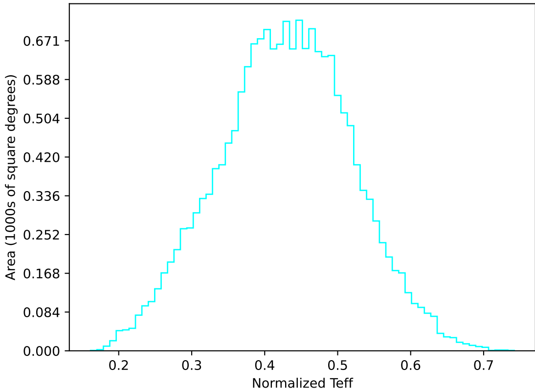
too_elab_heavy_r64_d2_griz_v3.4_10yrs WFD u band: Normalized Teff
