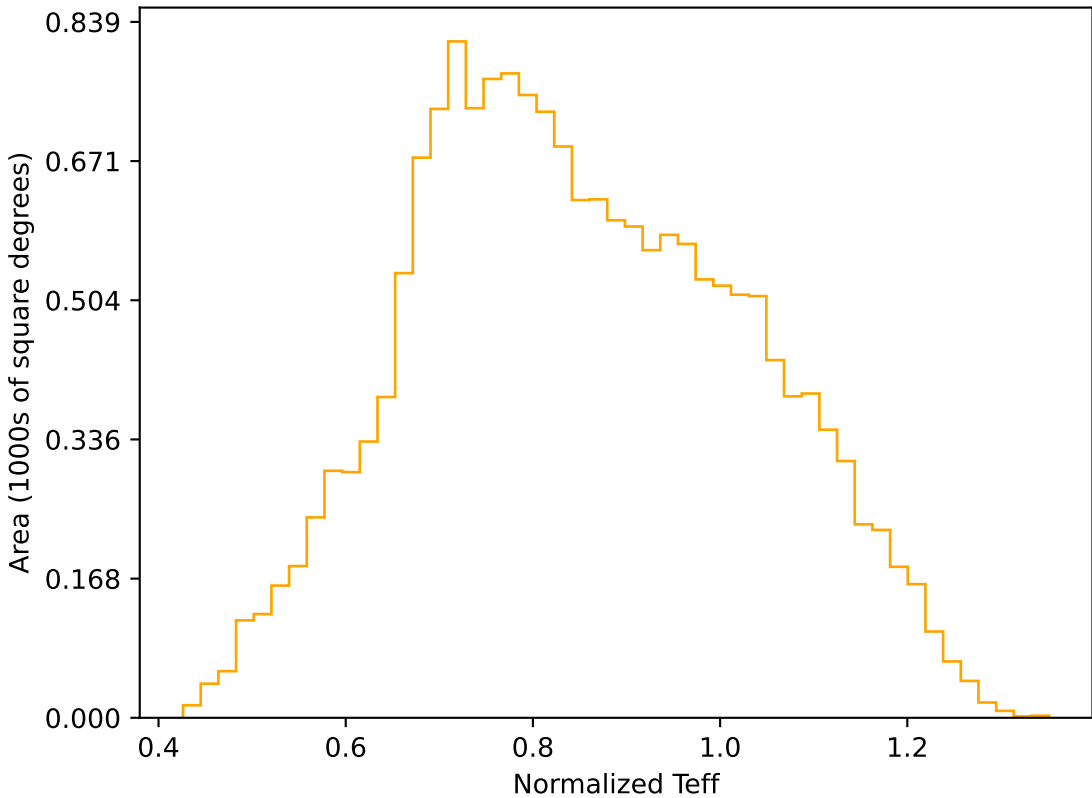
too_elab_heavy_r64_d2_griz_v3.4_10yrs WFD r band: Normalized Teff
