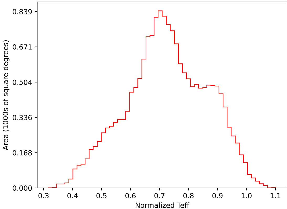
too_elab_heavy_r64_d2_griz_v3.4_10yrs WFD i band: Normalized Teff
