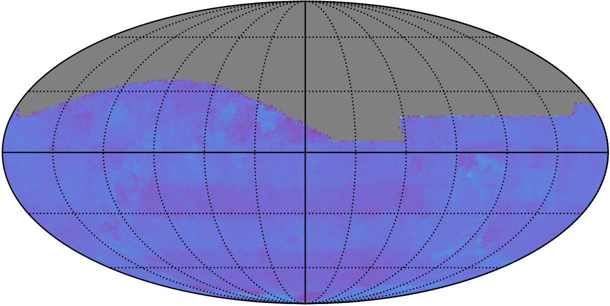
too_elab_heavy_r64_d2_griz_v3.4_10yrs All sky: Normalized Proper Motion Uncert @ 24.0
