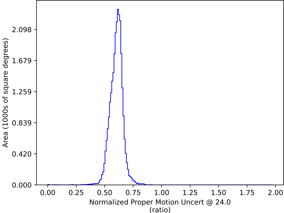
too_elab_heavy_r64_d2_griz_v3.4_10yrs All sky: Normalized Proper Motion Uncert @ 24.0
