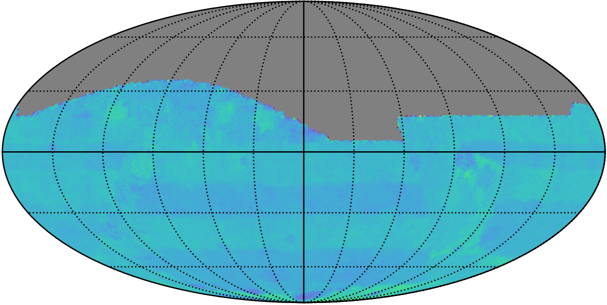
too_elab_heavy_r64_d2_griz_v3.4_10yrs All sky: Normalized Proper Motion Uncert @ 20.5
