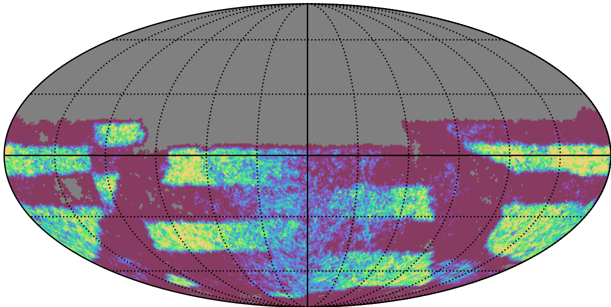
too_elab_heavy_r64_d2_griz_v3.4_10yrs Yr 3-4 y band: NVisits
