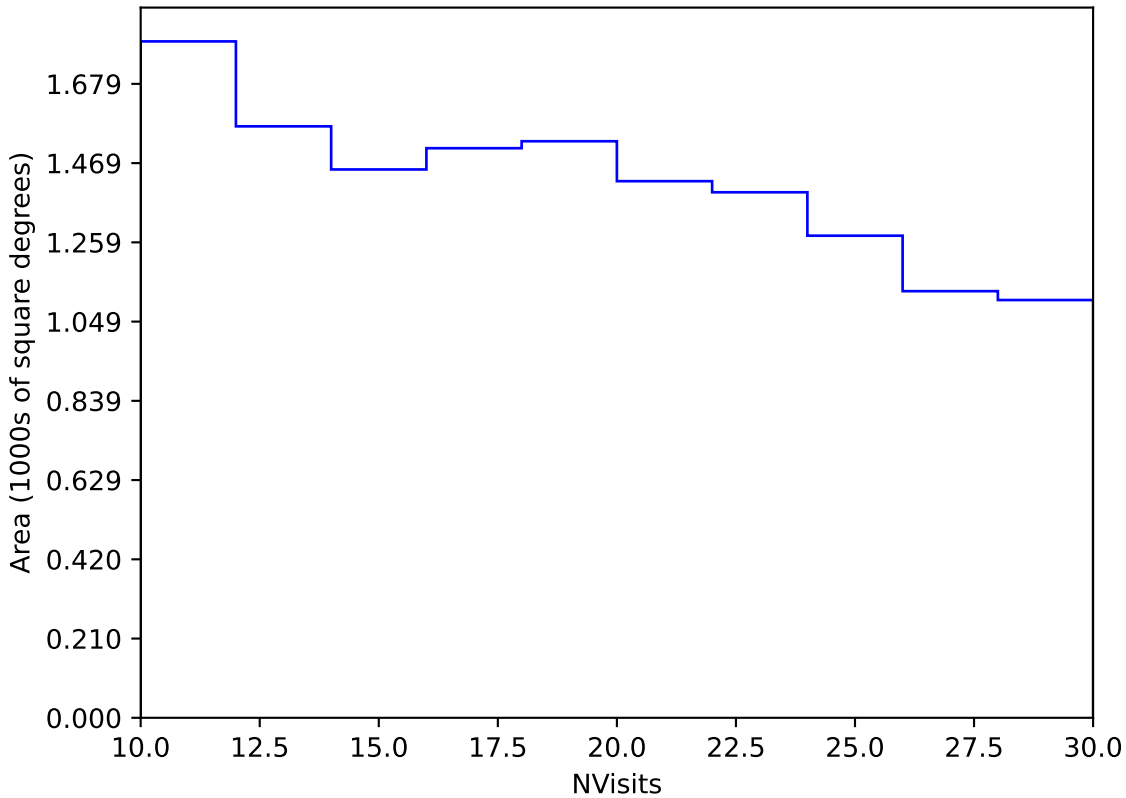
too_elab_heavy_r64_d2_griz_v3.4_10yrs Yr 3-4 y band: NVisits
