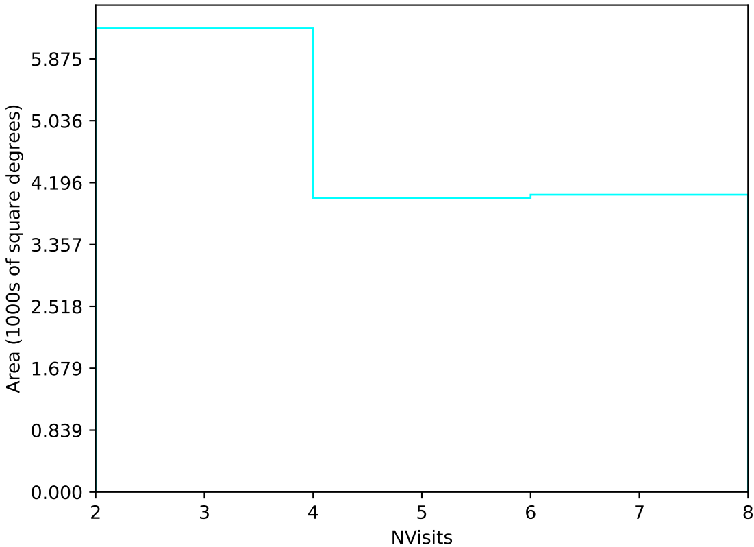
too_elab_heavy_r64_d2_griz_v3.4_10yrs Yr 3-4 u band: NVisits
