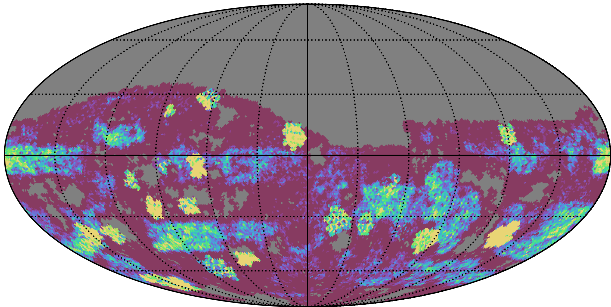
too_elab_heavy_r64_d2_griz_v3.4_10yrs Yr 3-4 g band: NVisits
