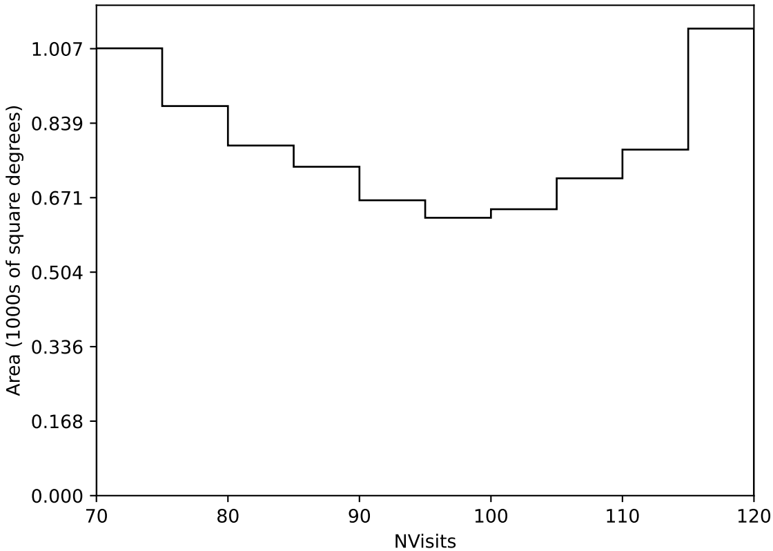
too_elab_heavy_r64_d2_griz_v3.4_10yrs Yr 3-4 all bands: NVisits
