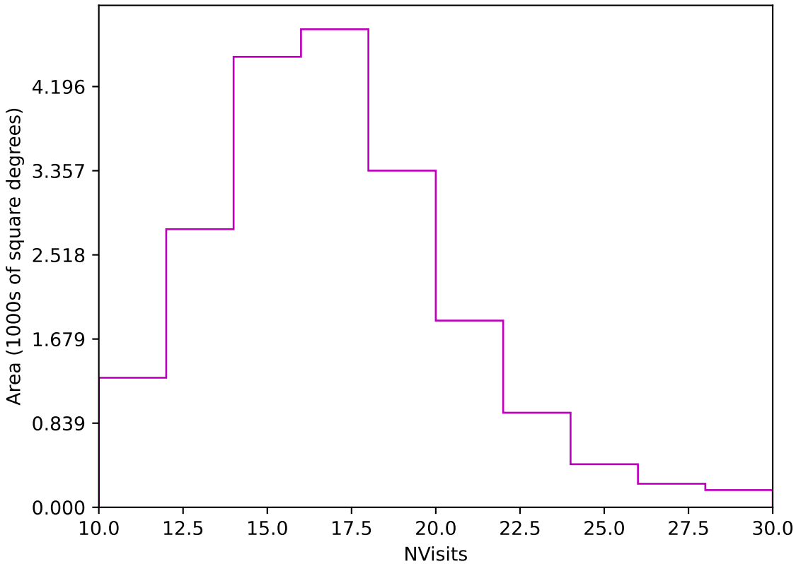
too_elab_heavy_r64_d2_griz_v3.4_10yrs Yr 1 z band: NVisits
