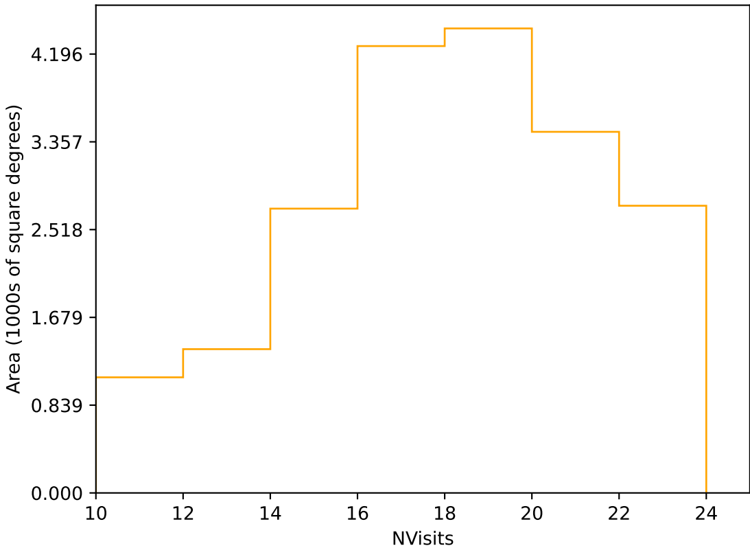
too_elab_heavy_r64_d2_griz_v3.4_10yrs Yr 1 r band: NVisits
