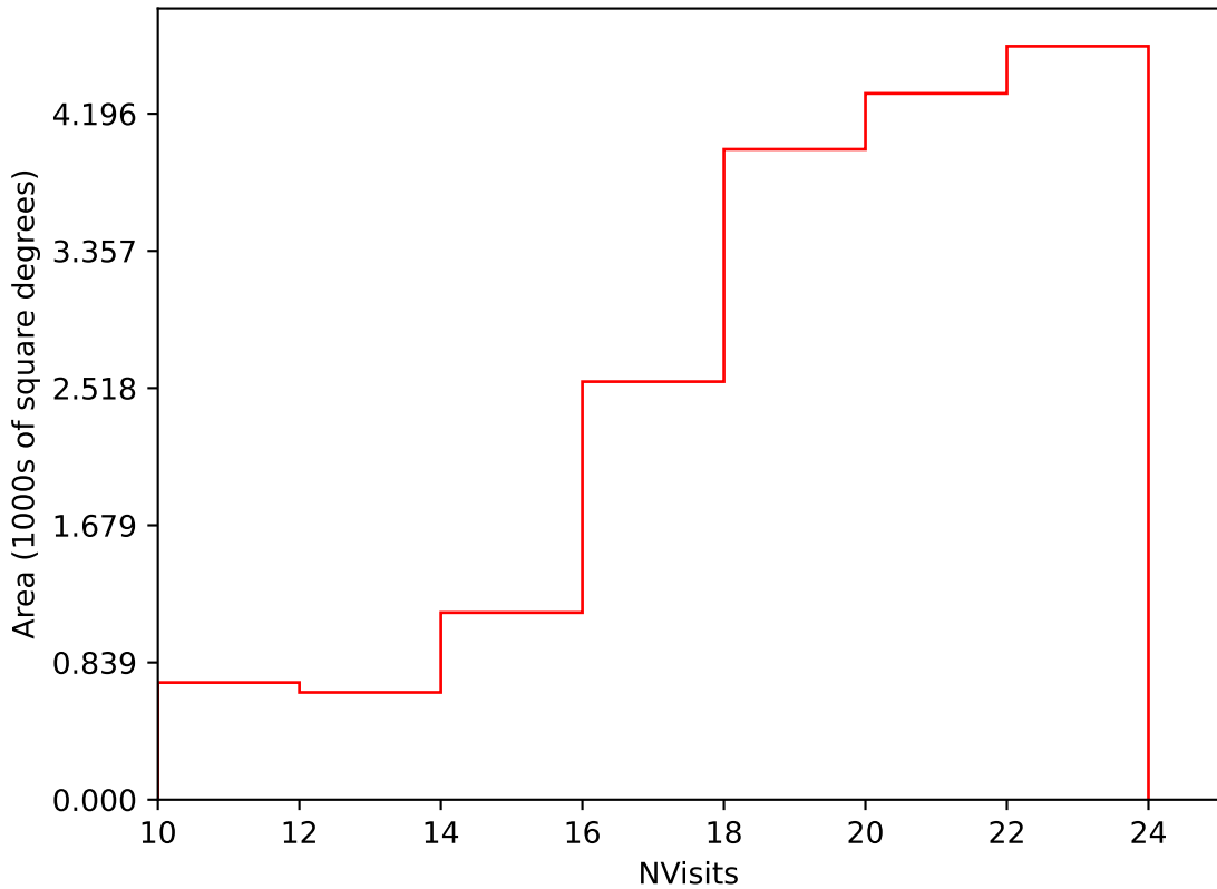
too_elab_heavy_r64_d2_griz_v3.4_10yrs Yr 1 i band: NVisits
