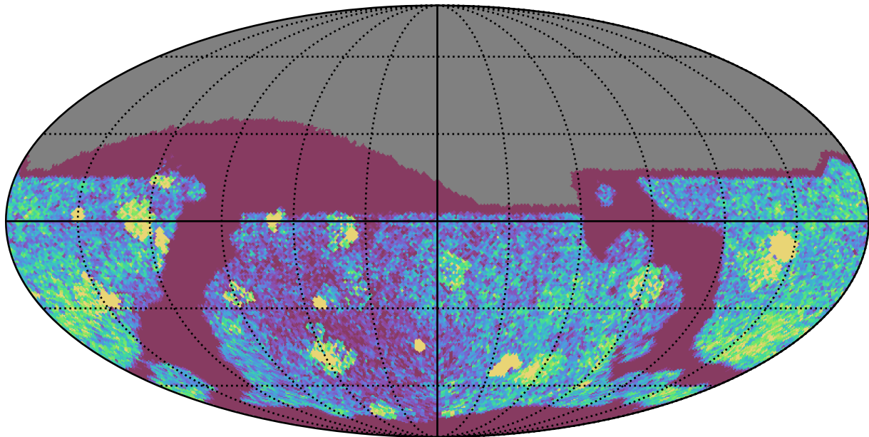
too_elab_heavy_r64_d2_griz_v3.4_10yrs Yr 1 all bands: NVisits
