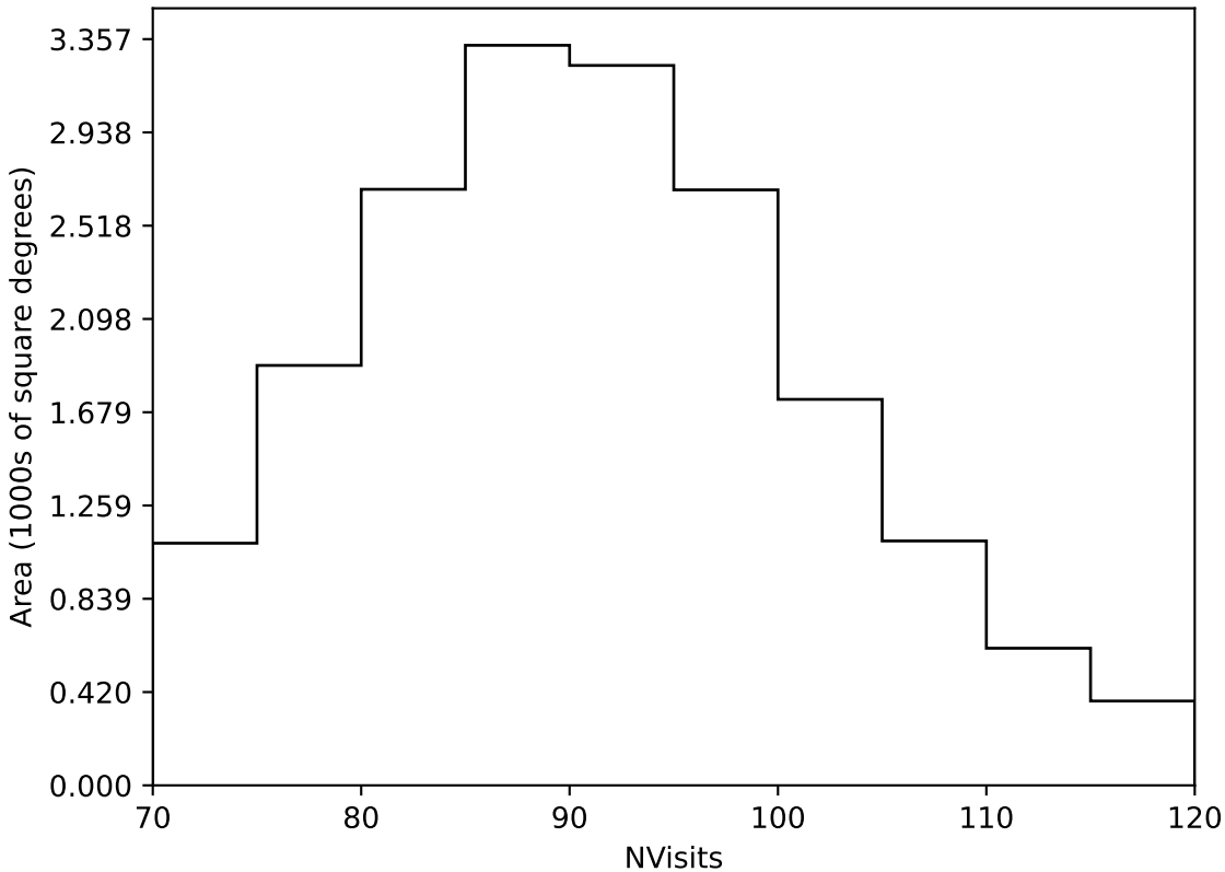
too_elab_heavy_r64_d2_griz_v3.4_10yrs Yr 1 all bands: NVisits
