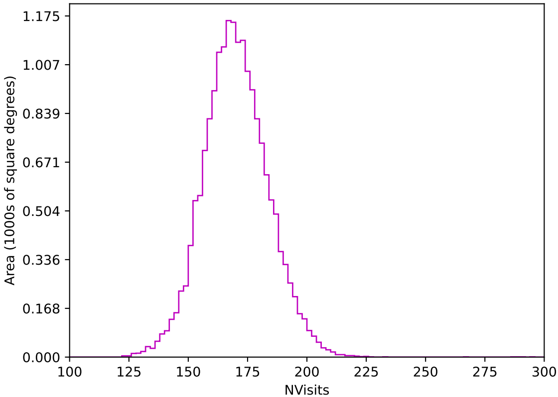
too_elab_heavy_r64_d2_griz_v3.4_10yrs WFD z band: NVisits
