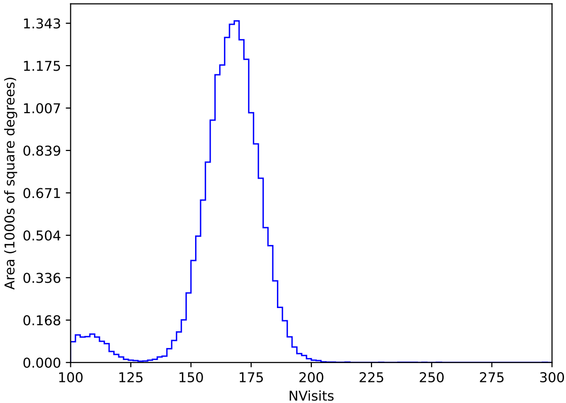
too_elab_heavy_r64_d2_griz_v3.4_10yrs WFD y band: NVisits
