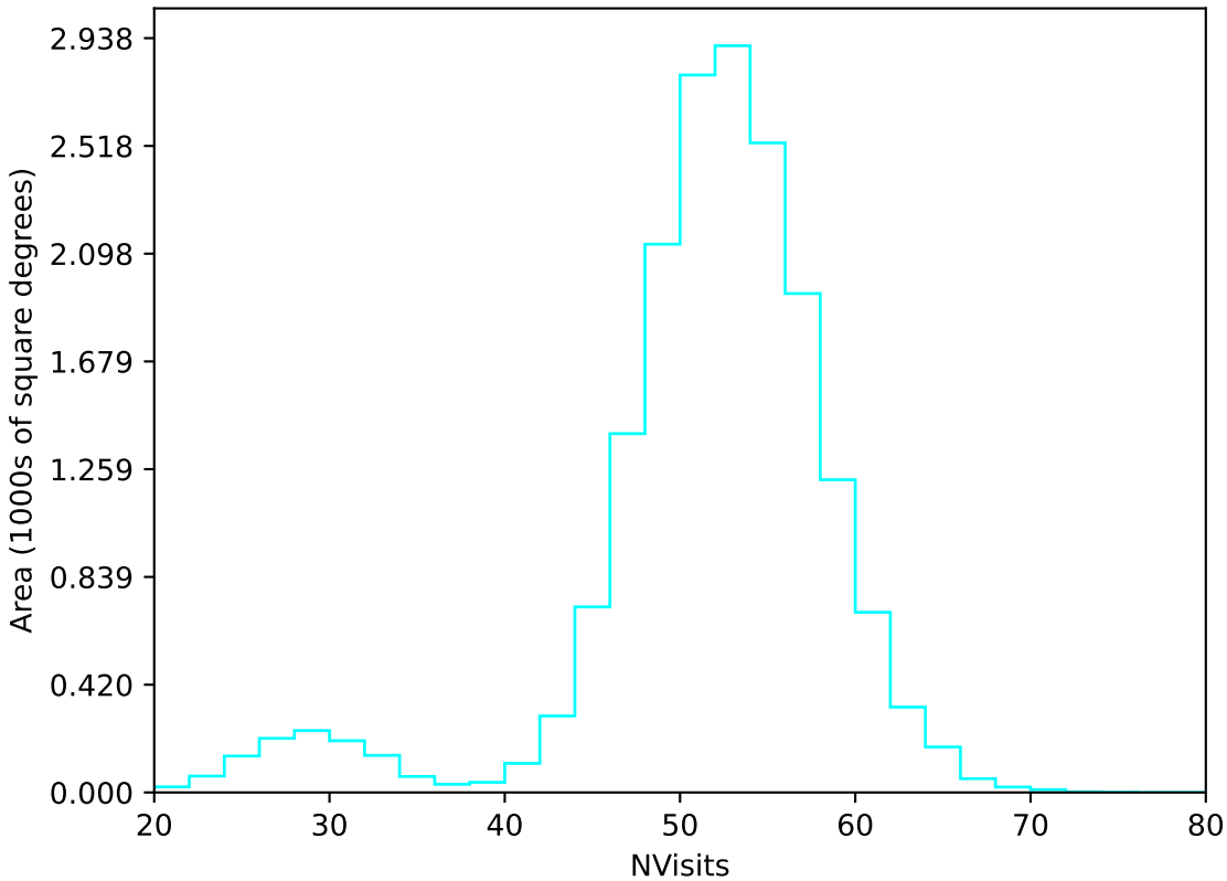
too_elab_heavy_r64_d2_griz_v3.4_10yrs WFD u band: NVisits
