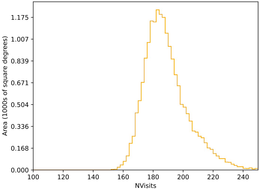
too_elab_heavy_r64_d2_griz_v3.4_10yrs WFD r band: NVisits
