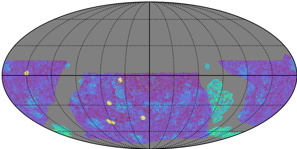
too_elab_heavy_r64_d2_griz_v3.4_10yrs WFD g band: NVisits
