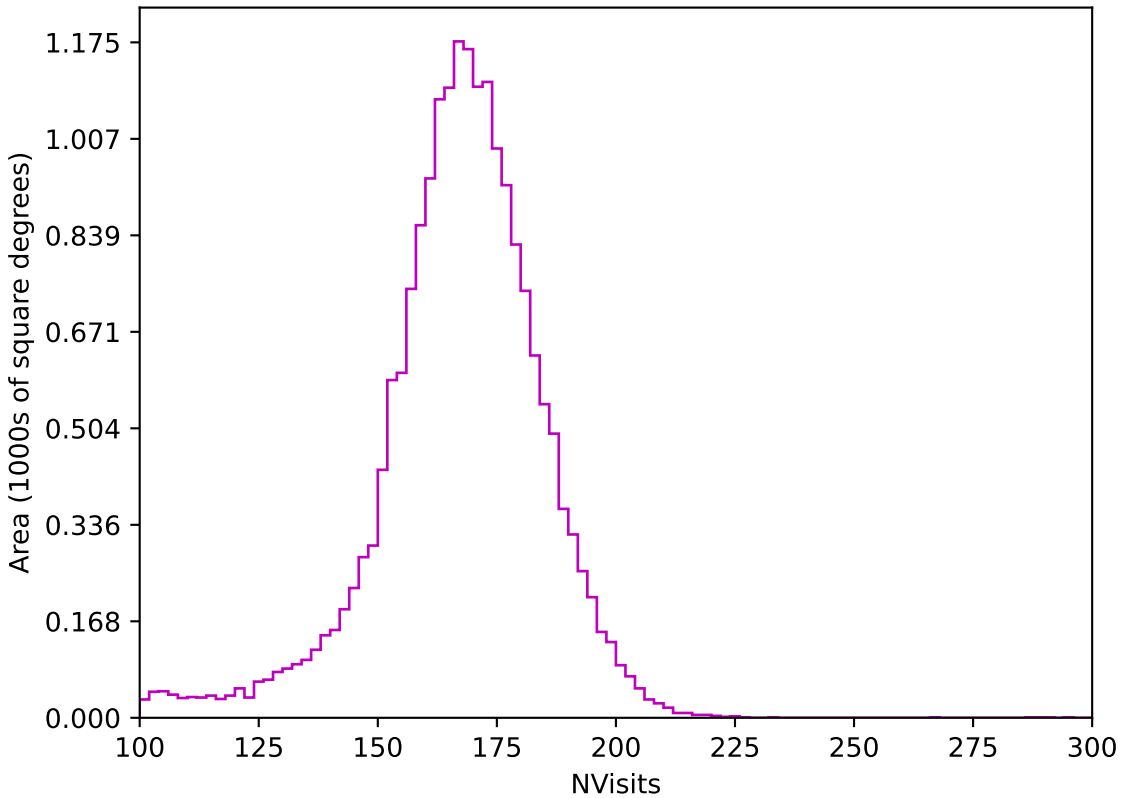
too_elab_heavy_r64_d2_griz_v3.4_10yrs All sky z band: NVisits
