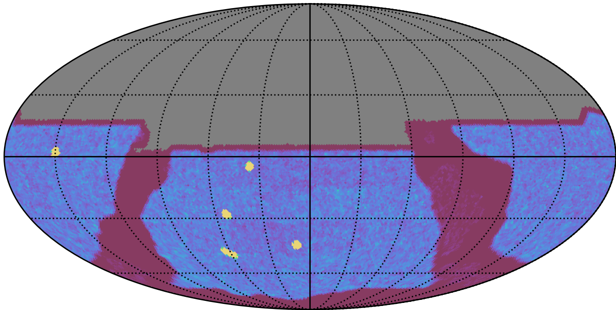
too_elab_heavy_r64_d2_griz_v3.4_10yrs All sky y band: NVisits
