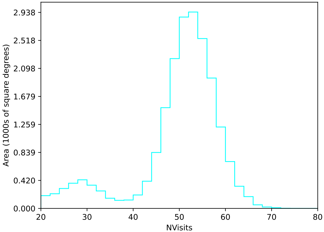
too_elab_heavy_r64_d2_griz_v3.4_10yrs All sky u band: NVisits
