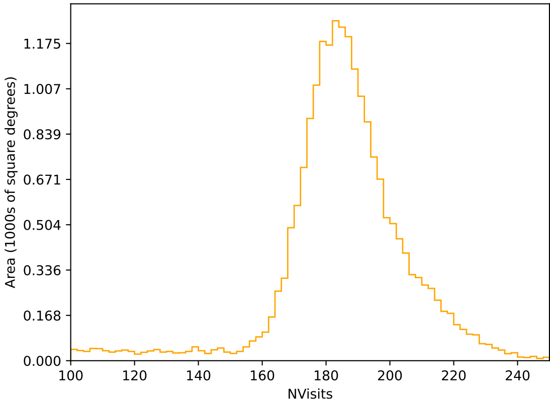
too_elab_heavy_r64_d2_griz_v3.4_10yrs All sky r band: NVisits
