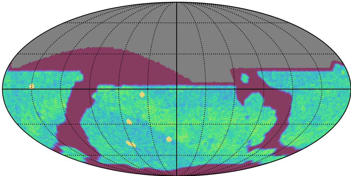
too_elab_heavy_r64_d2_griz_v3.4_10yrs All sky i band: NVisits
