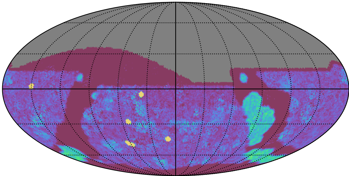
too_elab_heavy_r64_d2_griz_v3.4_10yrs All sky g band: NVisits
