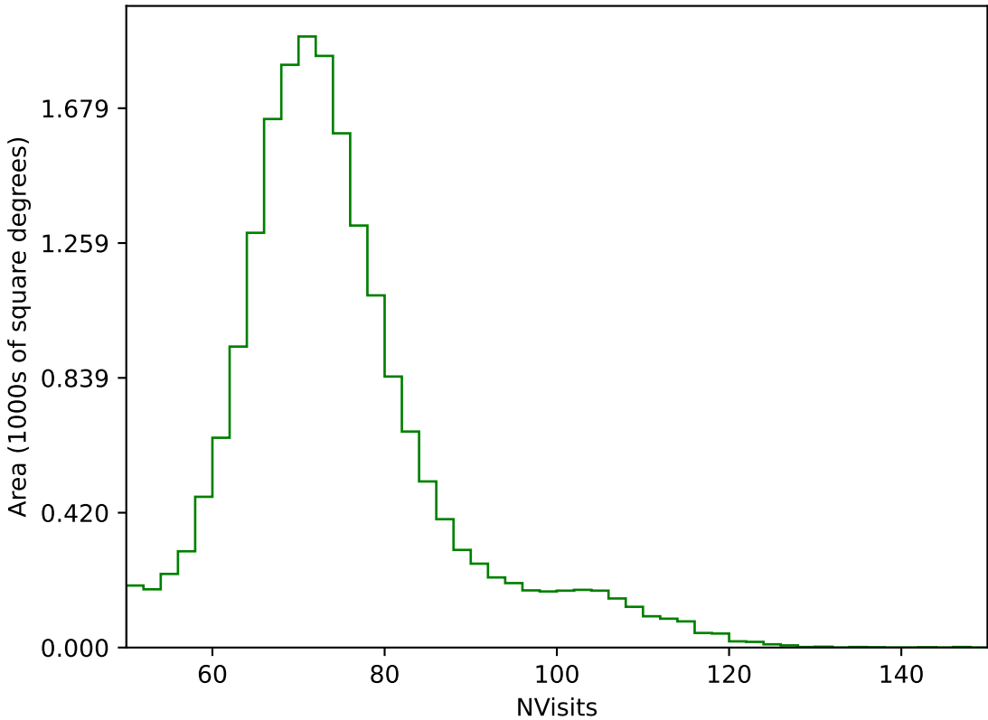
too_elab_heavy_r64_d2_griz_v3.4_10yrs All sky g band: NVisits
