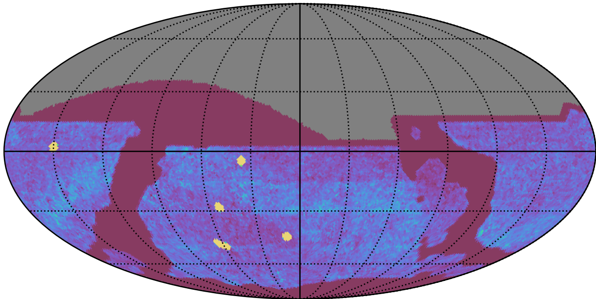
too_elab_heavy_r64_d2_griz_v3.4_10yrs All sky all bands: NVisits
