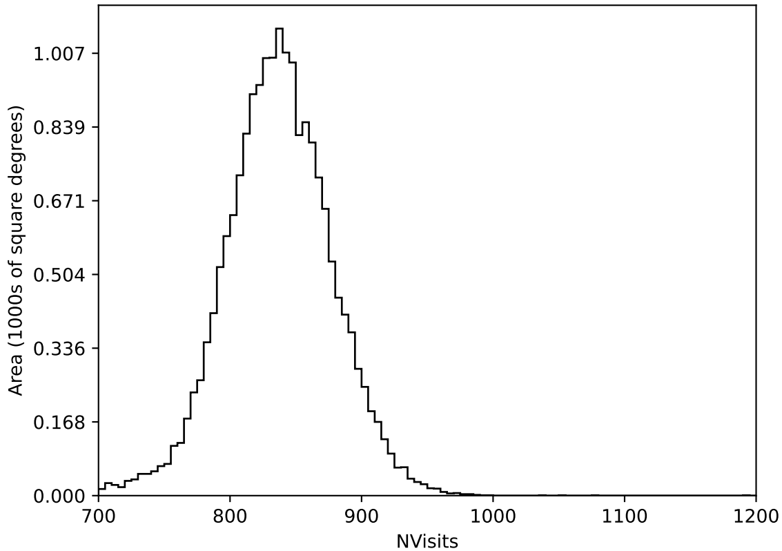
too_elab_heavy_r64_d2_griz_v3.4_10yrs All sky all bands: NVisits
