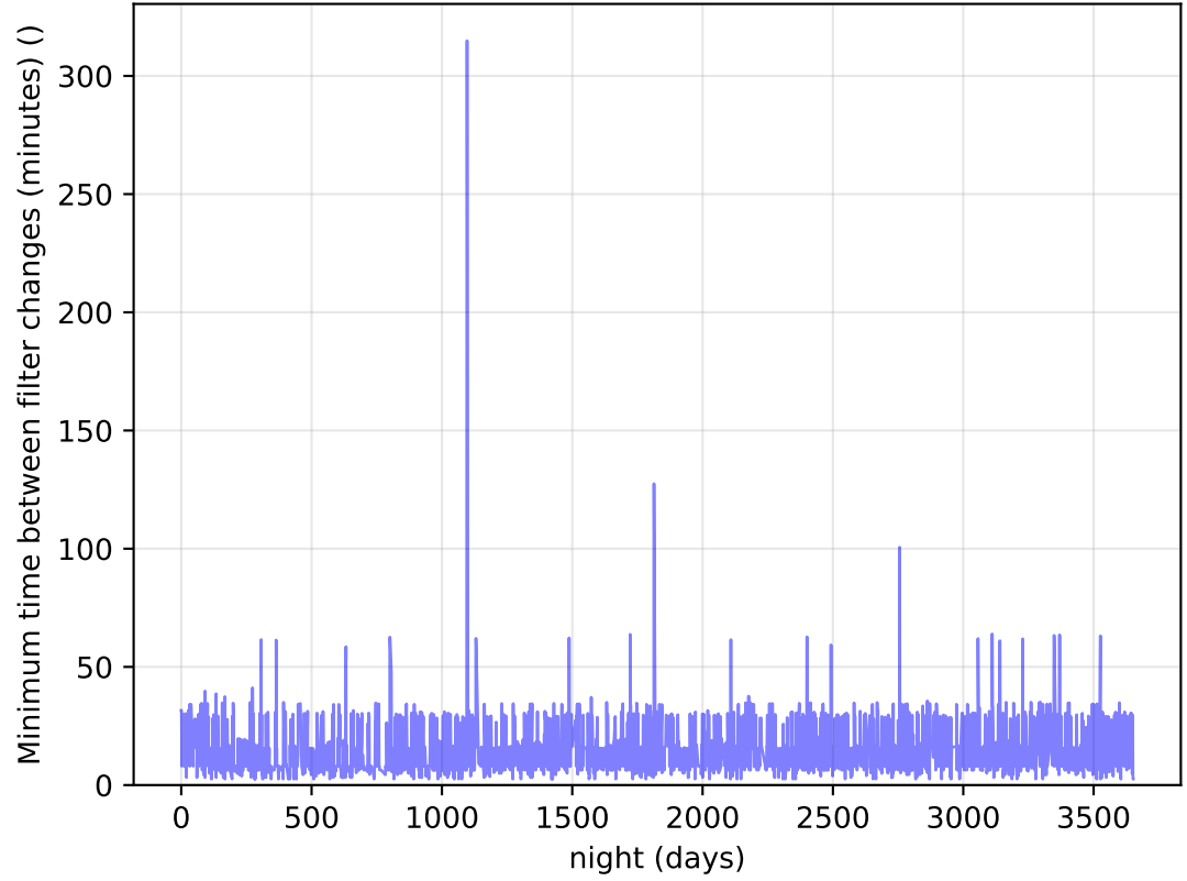
too_elab_heavy_r64_d2_griz_v3.4_10yrs Per Night: Minimum time between filter changes (minutes)
