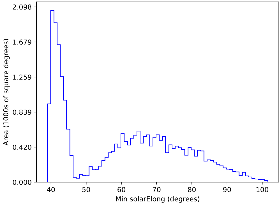
too_elab_heavy_r64_d2_griz_v3.4_10yrs All sky r band: Min solarElong
