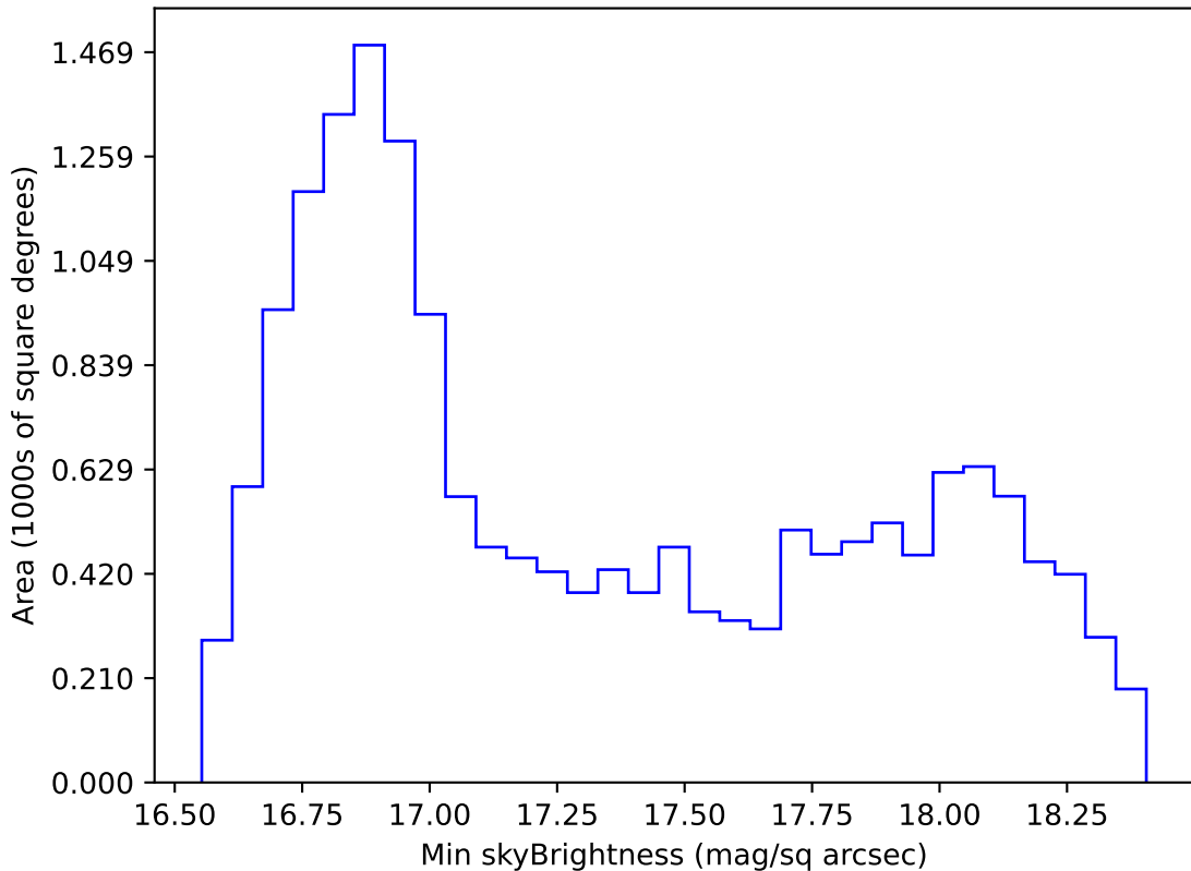
too_elab_heavy_r64_d2_griz_v3.4_10yrs WFD z band: Min skyBrightness
