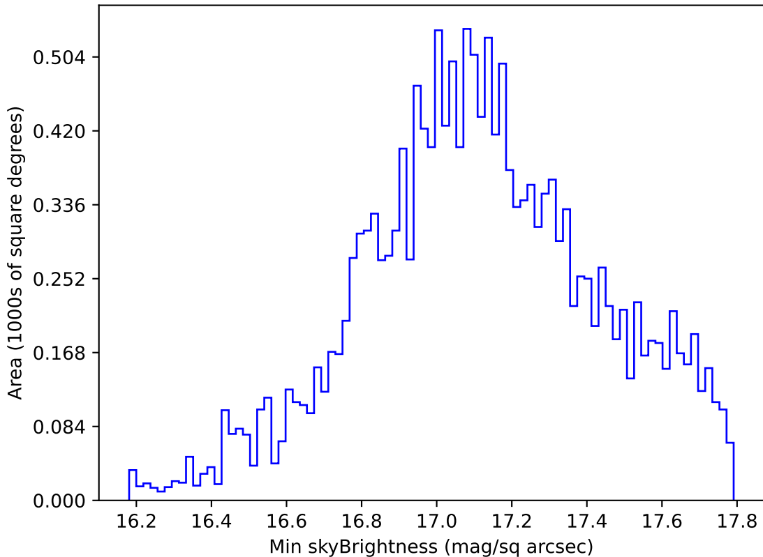
too_elab_heavy_r64_d2_griz_v3.4_10yrs WFD y band: Min skyBrightness
