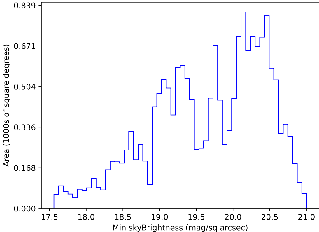
too_elab_heavy_r64_d2_griz_v3.4_10yrs WFD g band: Min skyBrightness
