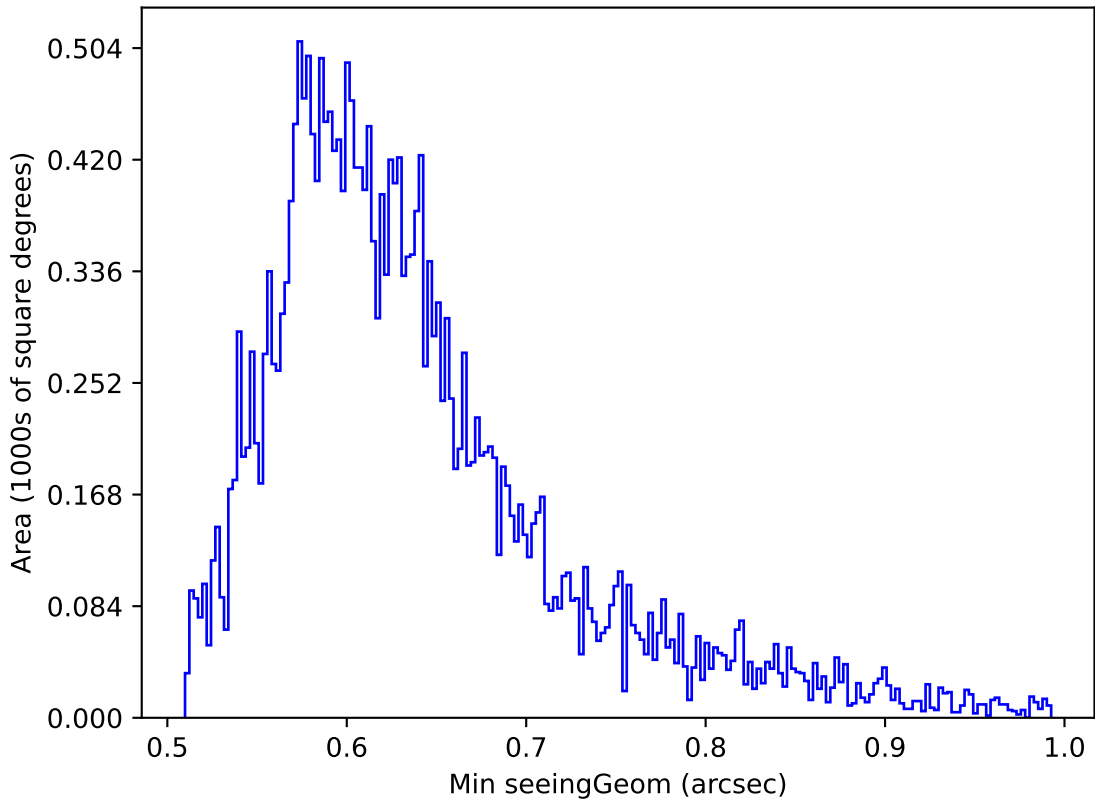
too_elab_heavy_r64_d2_griz_v3.4_10yrs Yr 1 z band: Min seeingGeom
