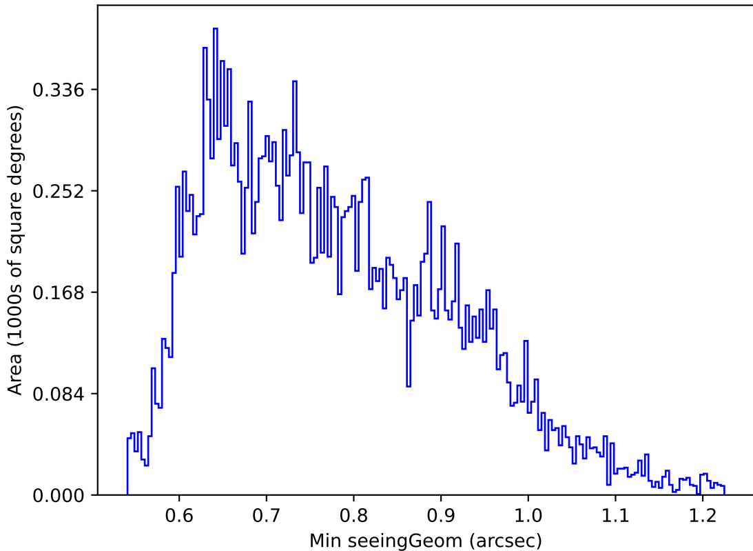
too_elab_heavy_r64_d2_griz_v3.4_10yrs Yr 1 u band: Min seeingGeom
