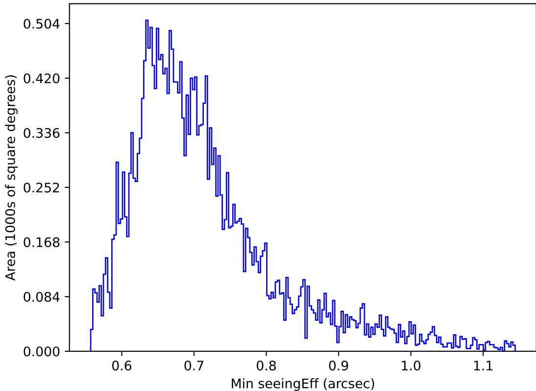
too_elab_heavy_r64_d2_griz_v3.4_10yrs Yr 1 z band: Min seeingEff
