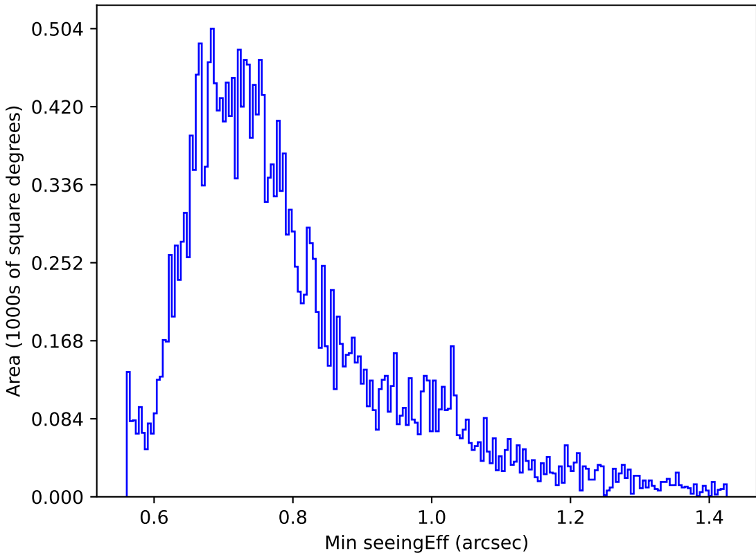
too_elab_heavy_r64_d2_griz_v3.4_10yrs Yr 1 g band: Min seeingEff
