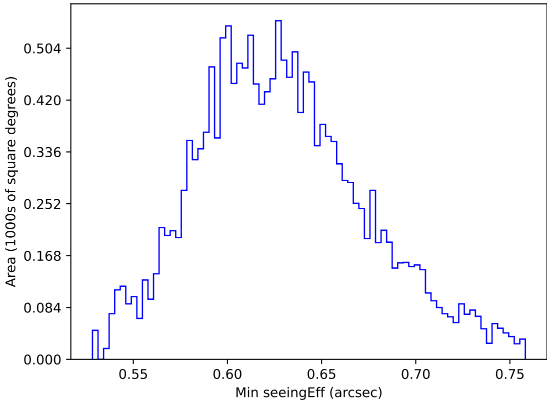
too_elab_heavy_r64_d2_griz_v3.4_10yrs WFD y band: Min seeingEff
