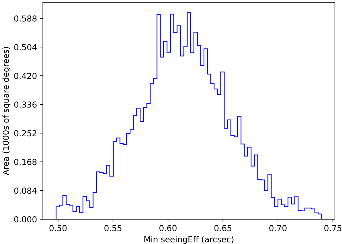
too_elab_heavy_r64_d2_griz_v3.4_10yrs WFD r band: Min seeingEff
