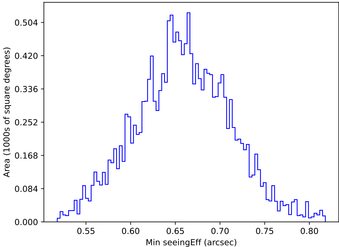
too_elab_heavy_r64_d2_griz_v3.4_10yrs WFD g band: Min seeingEff
