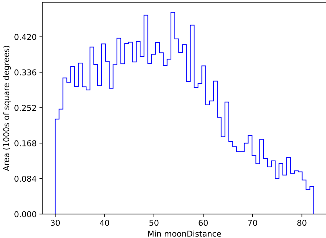
too_elab_heavy_r64_d2_griz_v3.4_10yrs WFD u band: Min moonDistance
