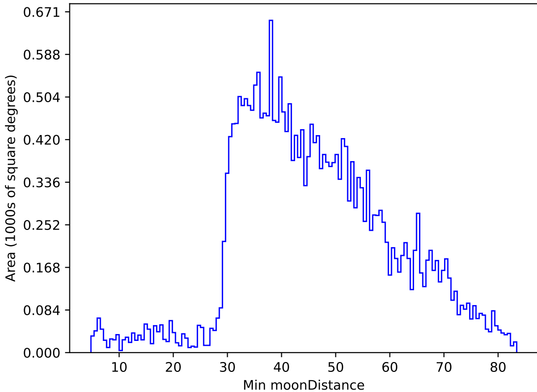
too_elab_heavy_r64_d2_griz_v3.4_10yrs All sky g band: Min moonDistance
