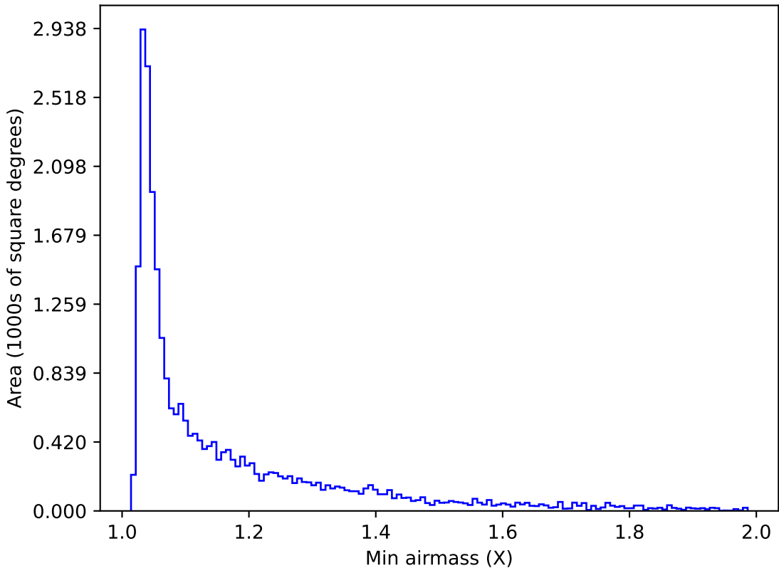
too_elab_heavy_r64_d2_griz_v3.4_10yrs Yr 1 i band: Min airmass
