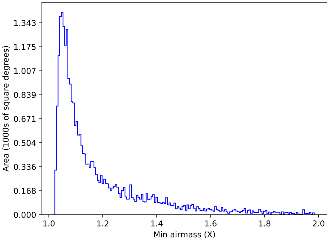
too_elab_heavy_r64_d2_griz_v3.4_10yrs Yr 1 g band: Min airmass
