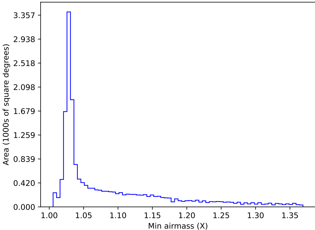
too_elab_heavy_r64_d2_griz_v3.4_10yrs WFD z band: Min airmass
