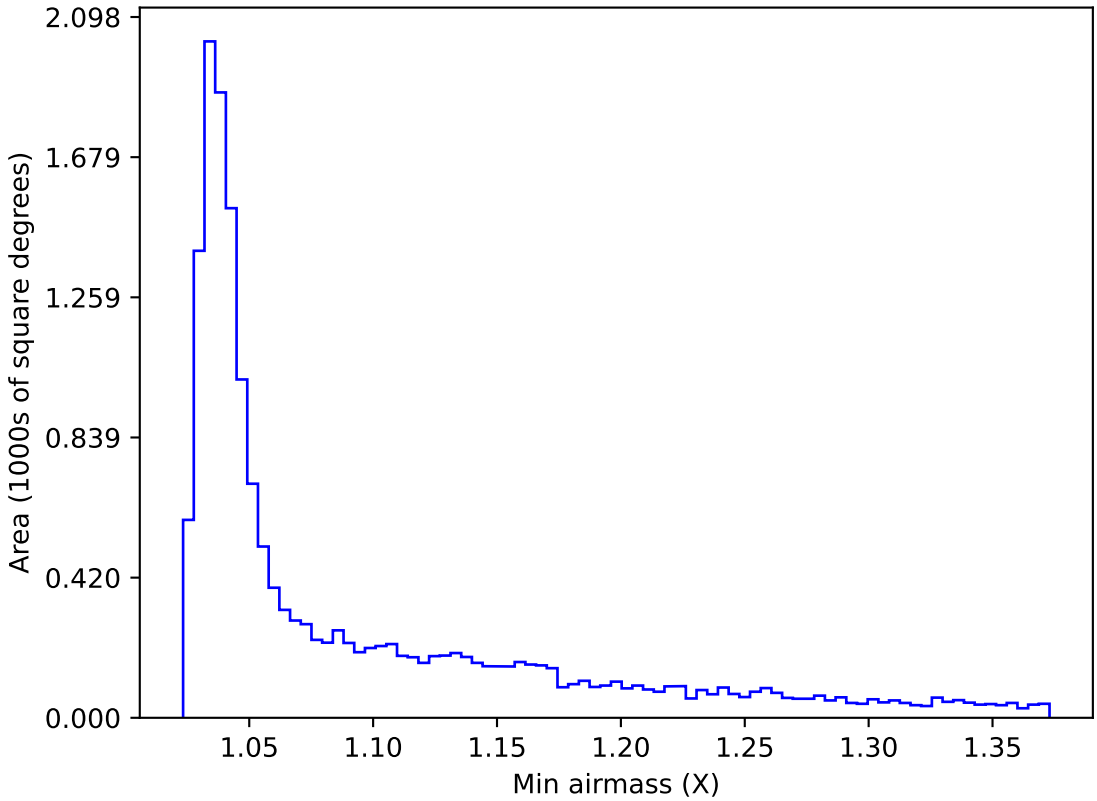
too_elab_heavy_r64_d2_griz_v3.4_10yrs WFD u band: Min airmass
