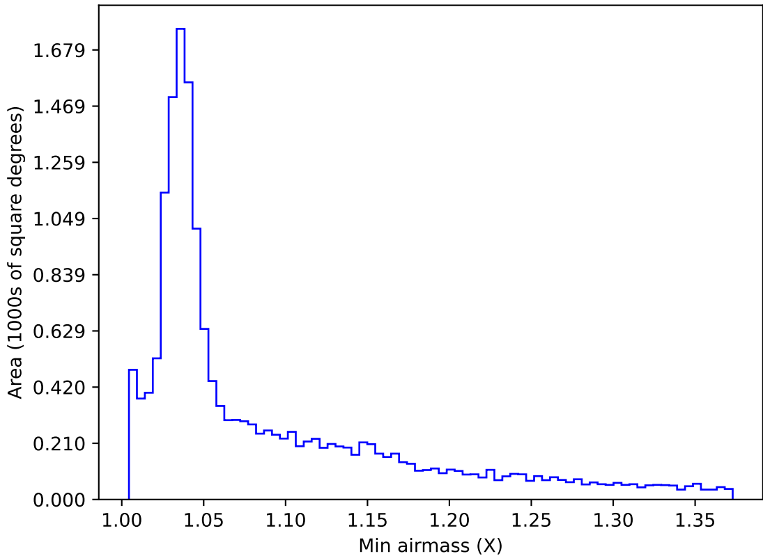
too_elab_heavy_r64_d2_griz_v3.4_10yrs WFD g band: Min airmass
