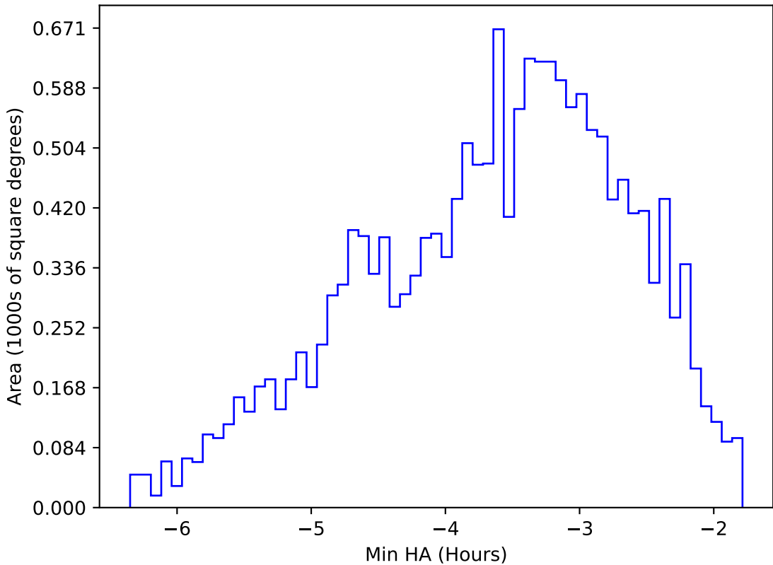
too_elab_heavy_r64_d2_griz_v3.4_10yrs WFD y band: Min HA
